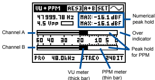
Fig 5-30, VU+PPM panel
