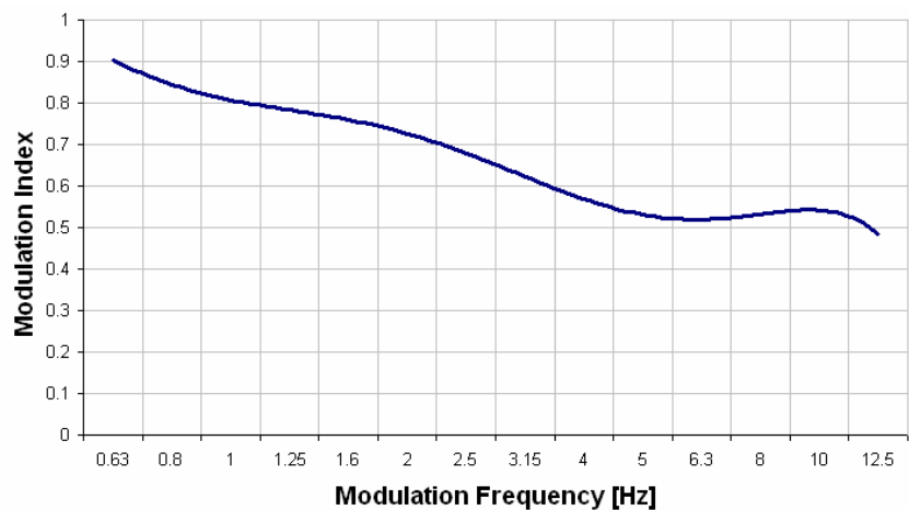
Figure 6: Modulation Transfer Function for one octave band
